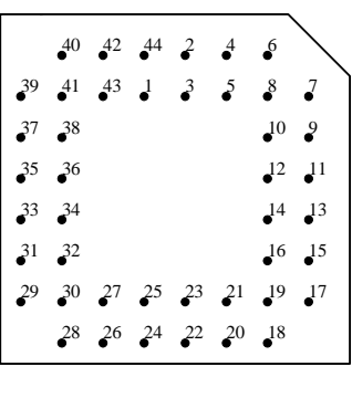
T89C51CC01 (bottom view)
